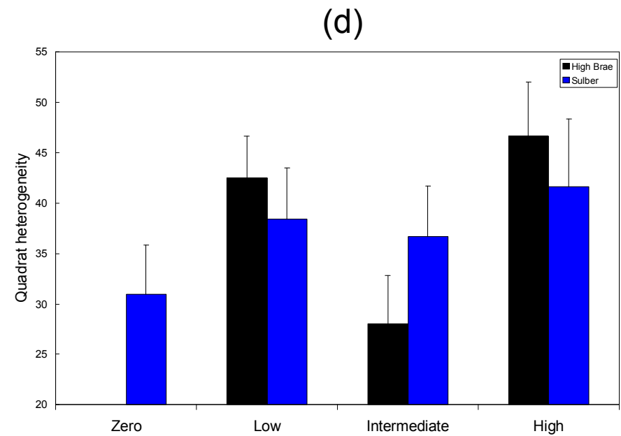
Figure 20. (a) Mean quadrat species richness, (b) Mean quadrat sward height, (c) Mean quadrat Shannon index and (d) Mean quadrat sward heterogeneity for each of the cattle activity zones in Sulber (blue) and High Brae (black). For all graphs, each column represents a mean and the vertical line +1 S.E.
