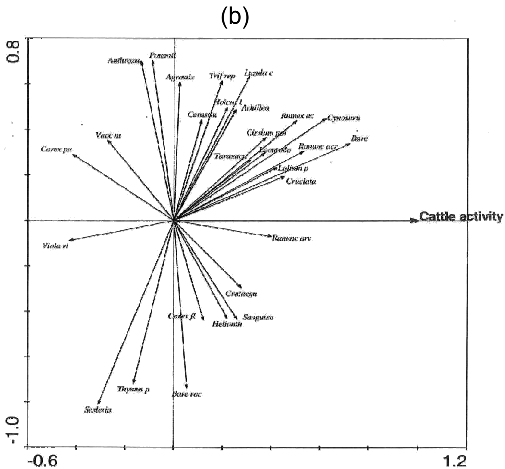
Figure 19. RDA ordination of species and the environmental variable of cattle activity (i.e. CA) for Sulber (a) and for High Brae (b). The X-axis indicates a relative index of association between species % cover values and cattle activity. The Y-axis represents variation not accounted for by cattle activity.
