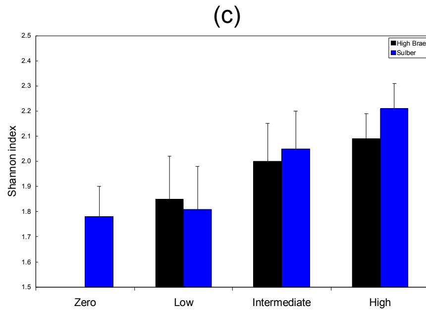
Figure 20. (a) Mean quadrat species richness, (b) Mean quadrat sward height, (c) Mean quadrat Shannon index and (d) Mean quadrat sward heterogeneity for each of the cattle activity zones in Sulber (blue) and High Brae (black). For all graphs, each column represents a mean and the vertical line +1 S.E.
